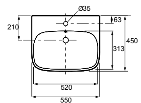
Top View (One Taphole shown)
