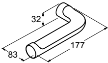
Isometric View
