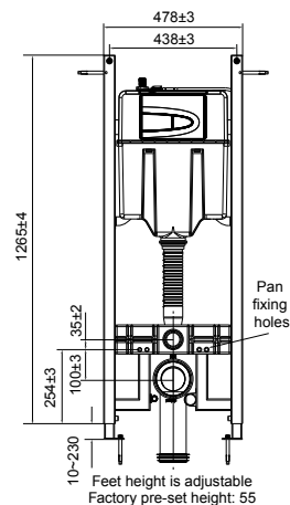
In Wall View
