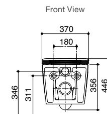
In Wall Views – Slim
