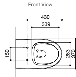
In Wall Views – Slim
