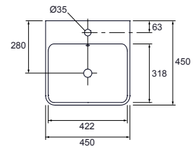
Top View (One Taphole shown)
