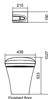
In Wall View
