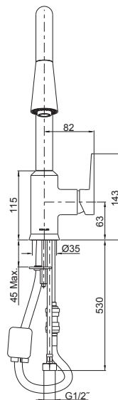
Front View
