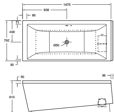
Rectangular Freestanding BubbleMassage Bath 18344A-GAB-0
